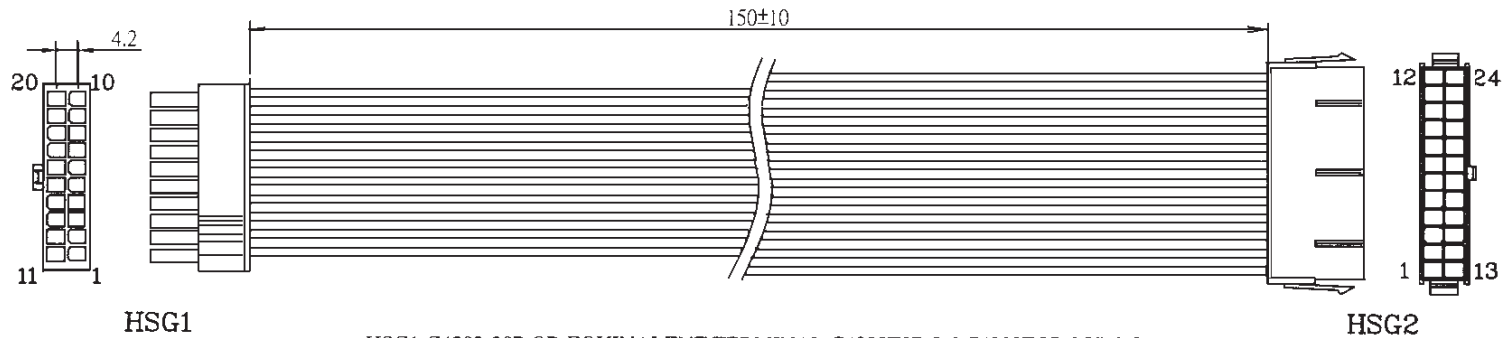
HSG1: C4202-20P OR EQUIVALENT, TERMINAL: C4202T2P-2 & C4202TOP-2OR EQUIVALENT. HSG2: JP2016-24 OR EQUIVALENT, TERMINAL: J2016BS-2OR EQUIVALENT.
