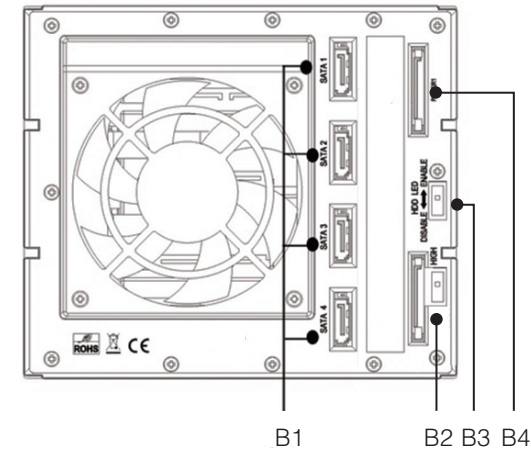
7pin SATA Edition Rear View
