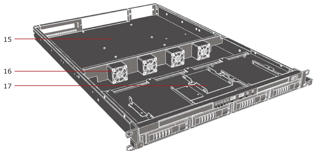
Top View
