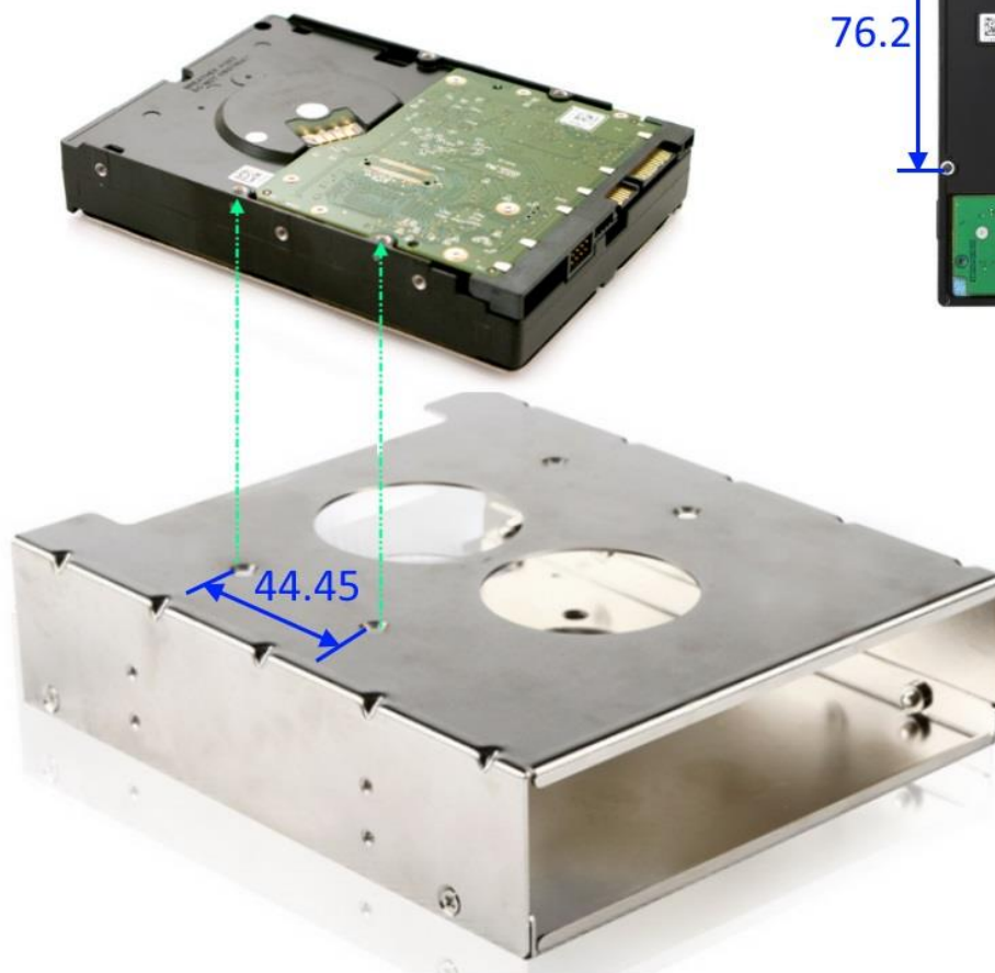
SFF-8301 specification
