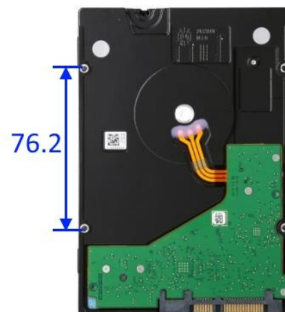
SFF-8301 specification
